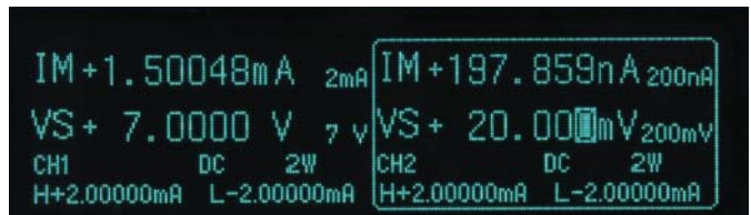
2-channel display example (256 x 64 dot matrix display)
